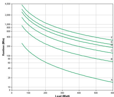
APC Smart-UPS X 750VA Rack/Tower LCD 230V (SMX750I)
