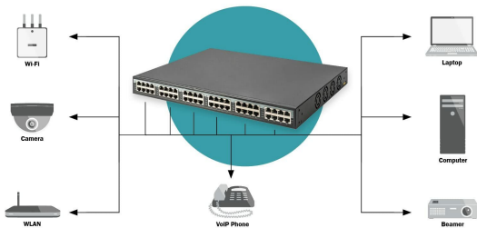
DN-95117 // 24 Port Gigabit Ethernet PoE+ Injector, 802.3af/at, 370 W
